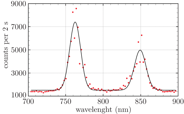
Figure 3.27: Spectral distribution of down-conversion light collected into a single-mode fibre. The solid line shows a Gaussian fit to the measured data. The photons of the pair are centered on the wavelengths of \lambda_1 \approx 763 nm and \lambda_2 \approx 849 nm, which agree well with the operation wavelengths of WDM. The lower peak number of counts at \lambda_2 is attributed to a reduced efficiency of the spectrometer towards NIR wavelengths and the offset of \approx 1100 counts is due to dark counts of the APDs.
