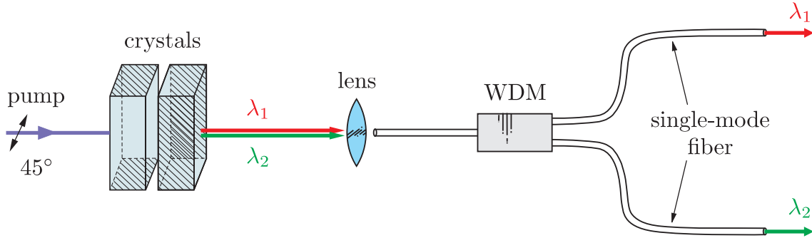
Figure 3.12: Conceptual layout of the method to generate entangled photon pairs using collinear geometry of SPDC operated in type I non-degenerate configuration.
